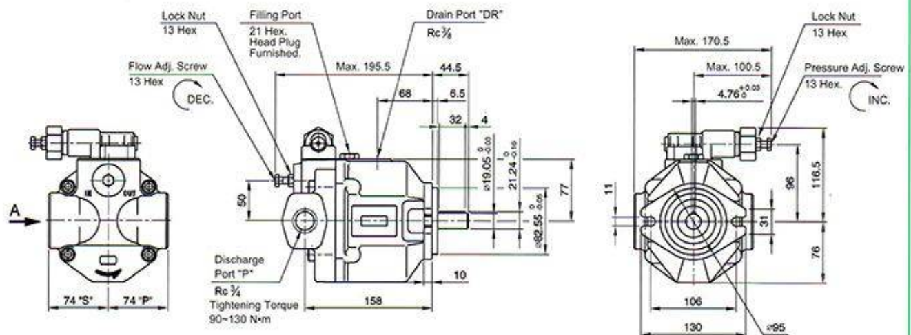
View A
