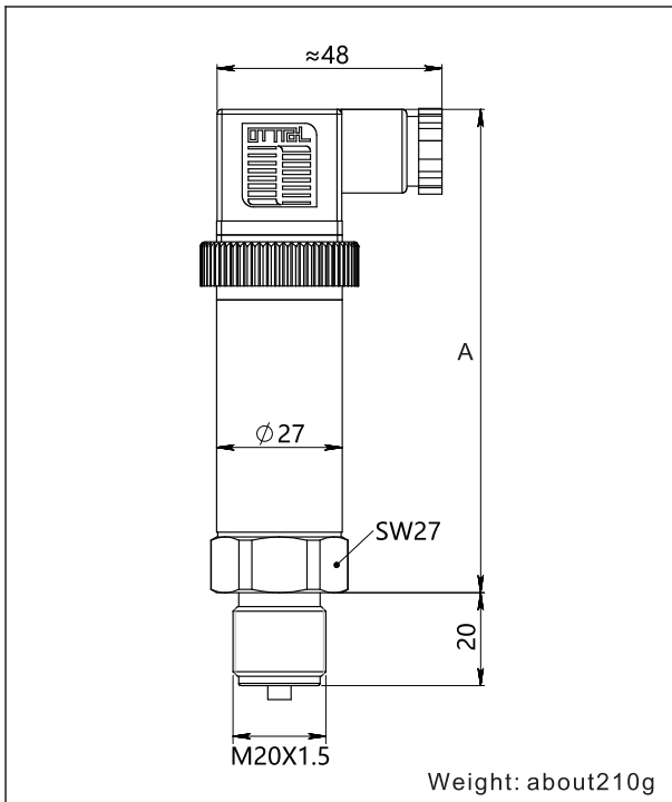
Value of A in different output signal types(DIN43650 adaptor)
