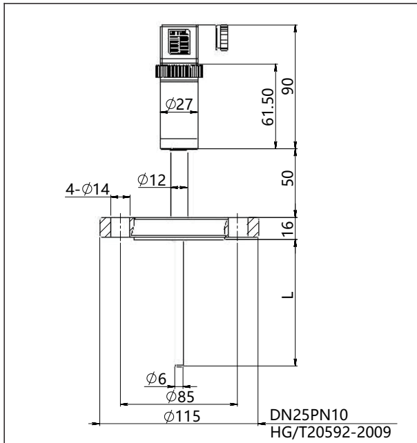
Process connection(M01) (unit: mm)
