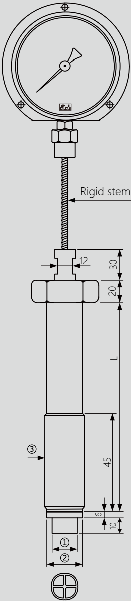
Rigid stem with capillary extension
