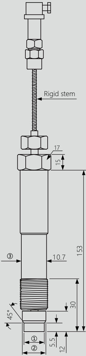
Rigid stem with capillary extension (pressure transmitter)
