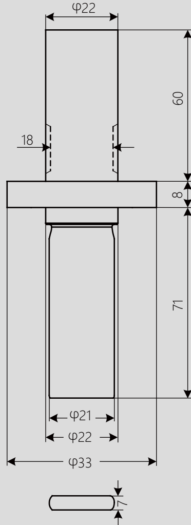
Fishtail seal type
