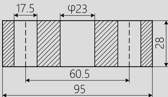
Retainer flange (mounting block or sealing block)
