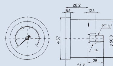
D-Type Dia. 2"
