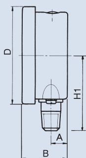
A-Type Dia. 2-1/2", 4"
