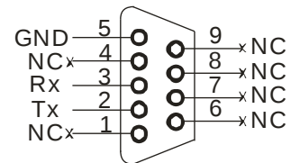
Female DB9 connector ↔ Female DB9 connector
