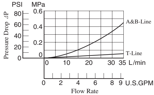
Pressure Drop
