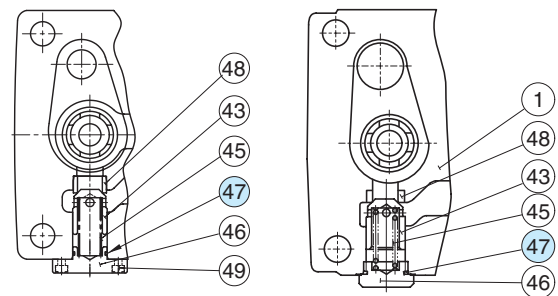
(FHCG-06 Type)
