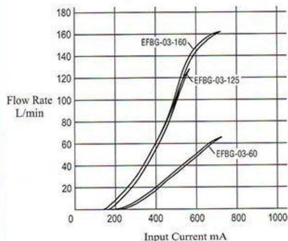
EFBG-*-20T145 Input Current vs. Flow
