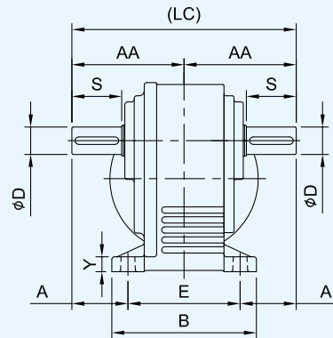
雙軸 DOUBLE SHAFT
