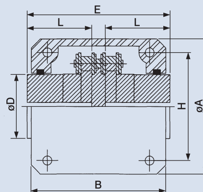
HT-Roller chain flexible coupling
