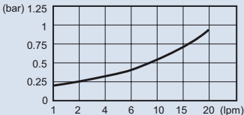
LOSS OF PRESSURE (at 32 Cst)
