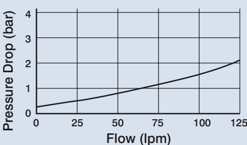
RG-06, RCG-06, RT-06, RCT-06
