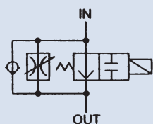
SINGLE TYPE
