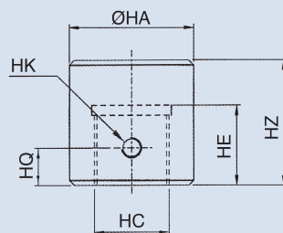
H type adaptor for welding
