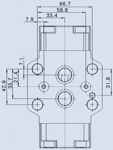
RGM-03, RCGM-03, HGM-03, HCGM-03, CPDGM-03
