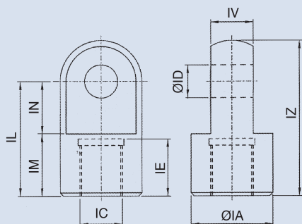
I type adaptor
