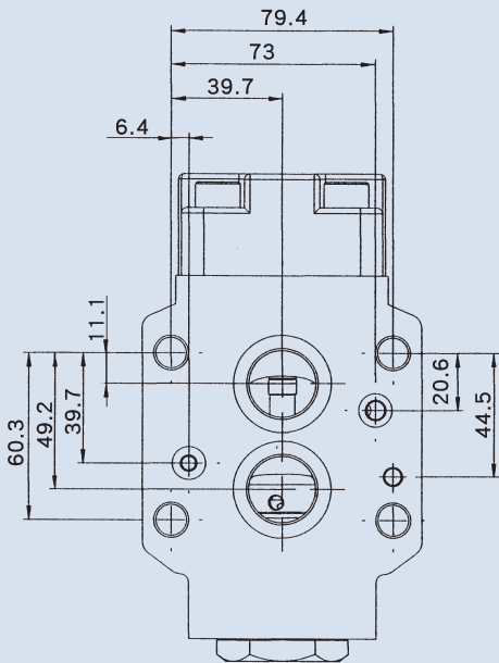
RGM-06, RCGM-06, HGM-06, HCGM-06, CPDGM-06
