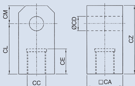
I type adaptor
