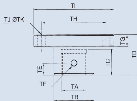
T type adaptor
