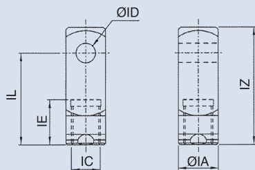
I type adaptor
