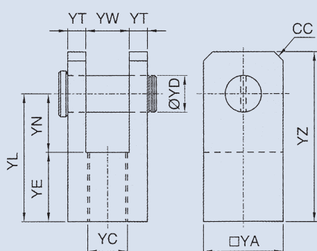
Y type adaptor with pin
